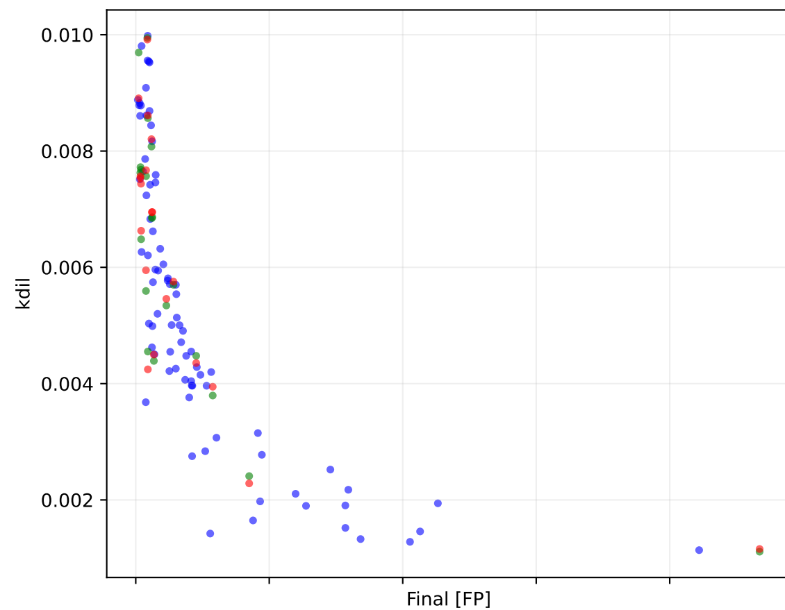
PILSTM Epoch 22000 lambda physics 0.0000
