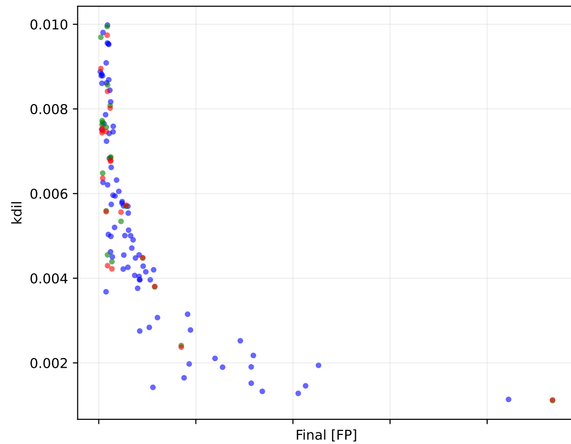
PILSTM Epoch 23000 lambda physics 0.0000
