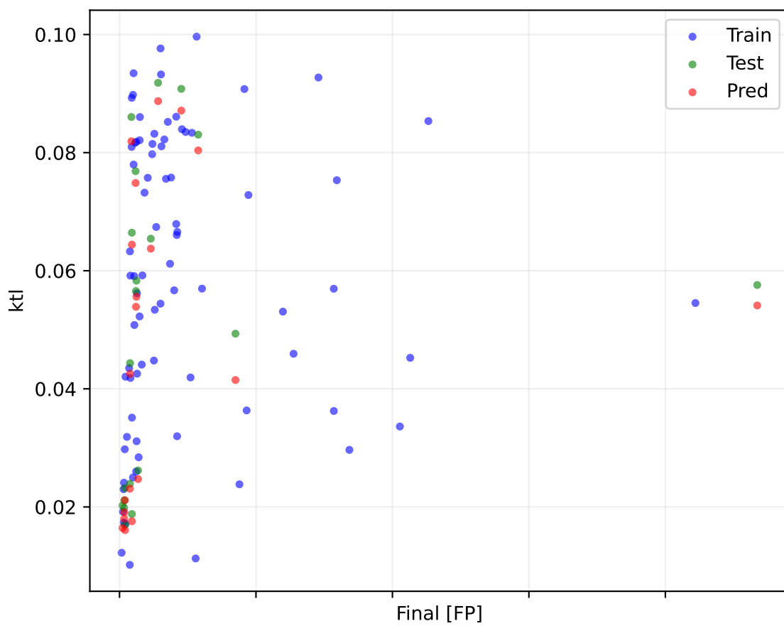
PILSTM Epoch 29000 lambda physics 0.0000
