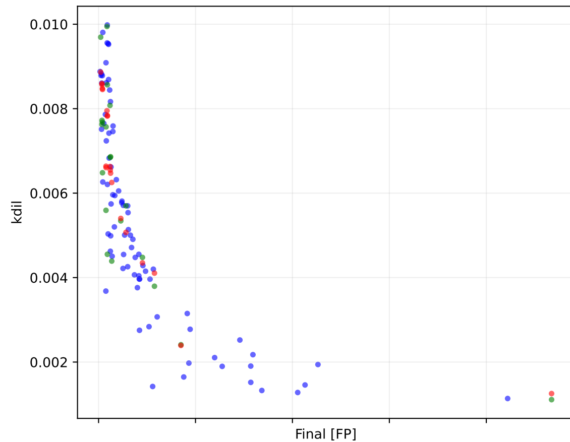
PILSTM Epoch 6000 lambda physics 0.0000
