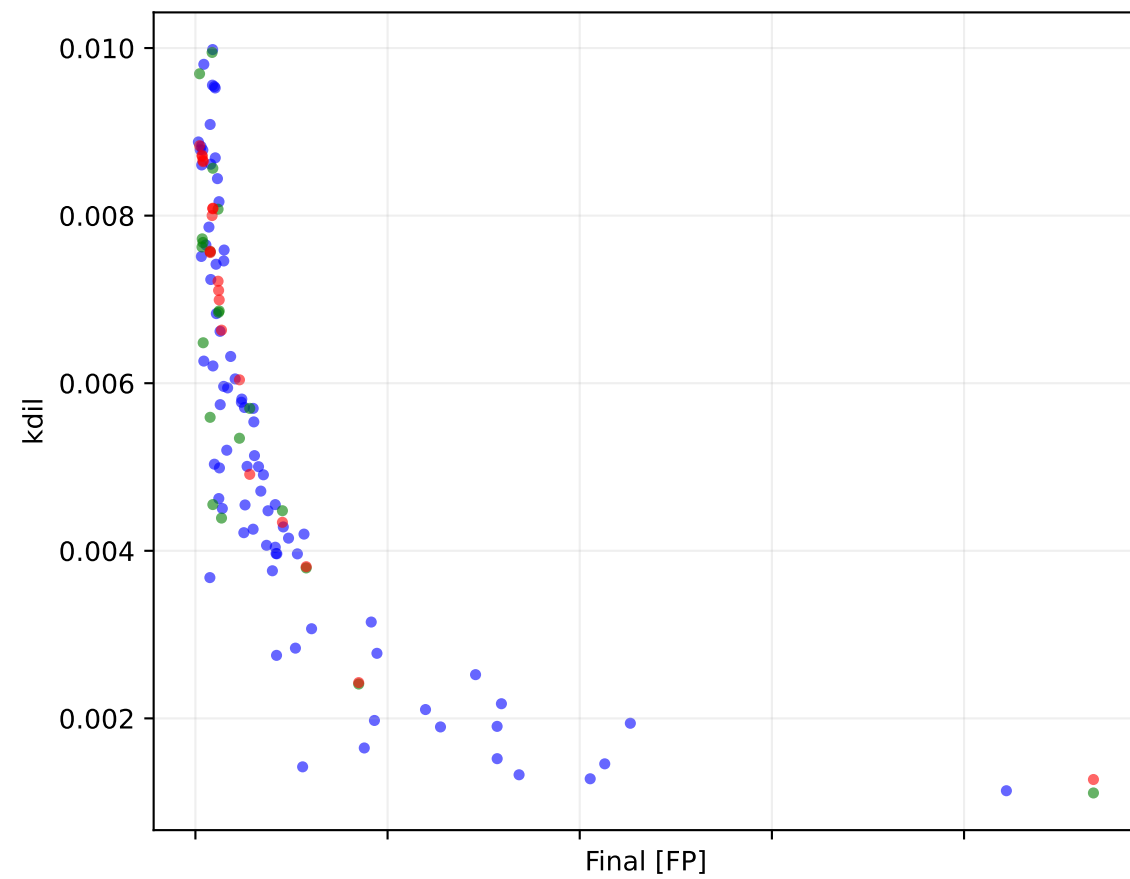
PILSTM Epoch 7000 lambda physics 0.0000
