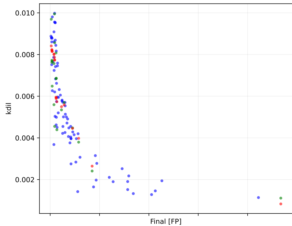
PILSTM Epoch 7000 lambda physics 0.0050
