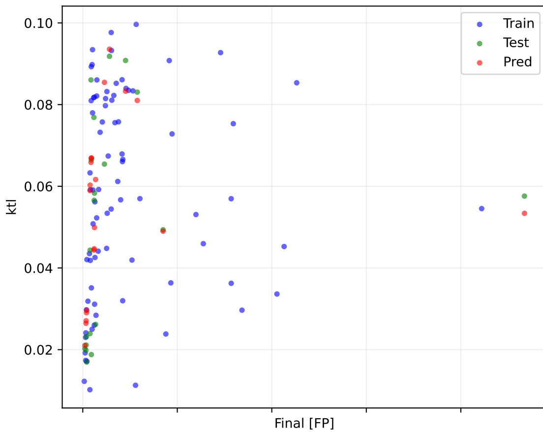
PILSTM Epoch 8000 lambda physics 0.0000
