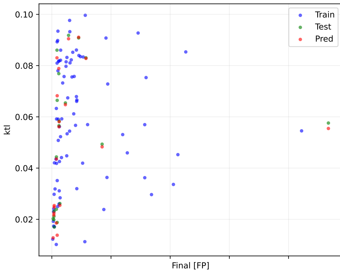
PILSTM Epoch 8000 lambda physics 0.0050
