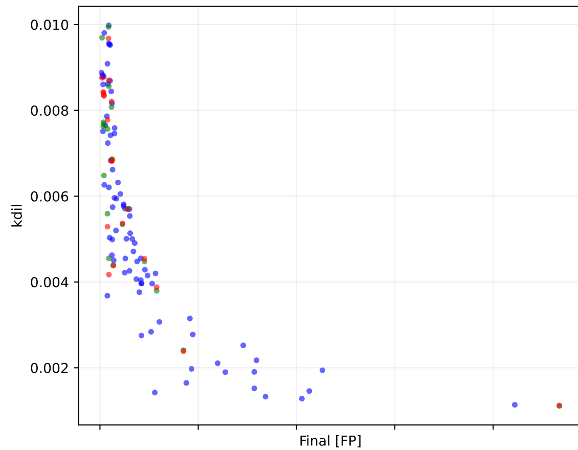
PILSTM Epoch 9000 lambda physics 0.0050
