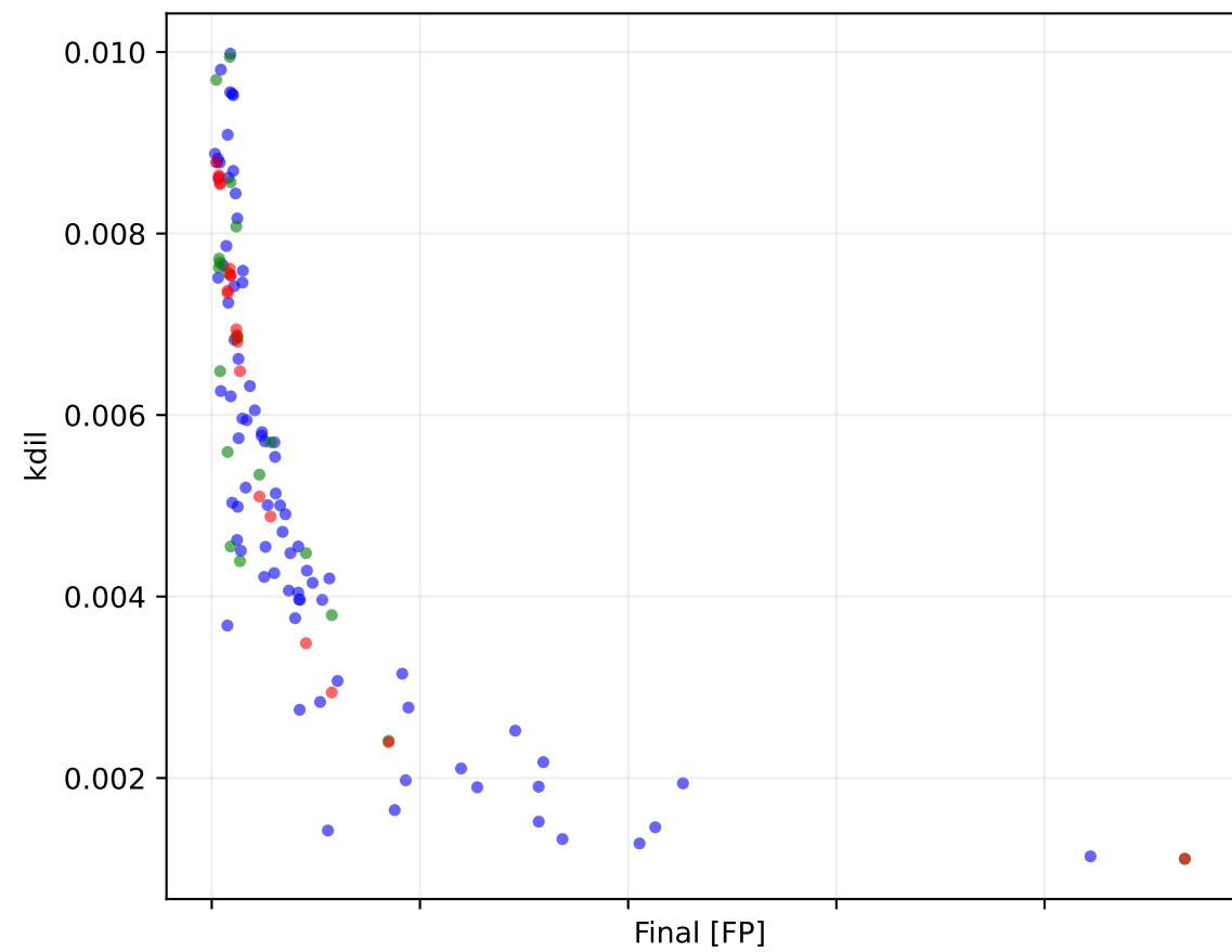
PILSTM Epoch 1000
