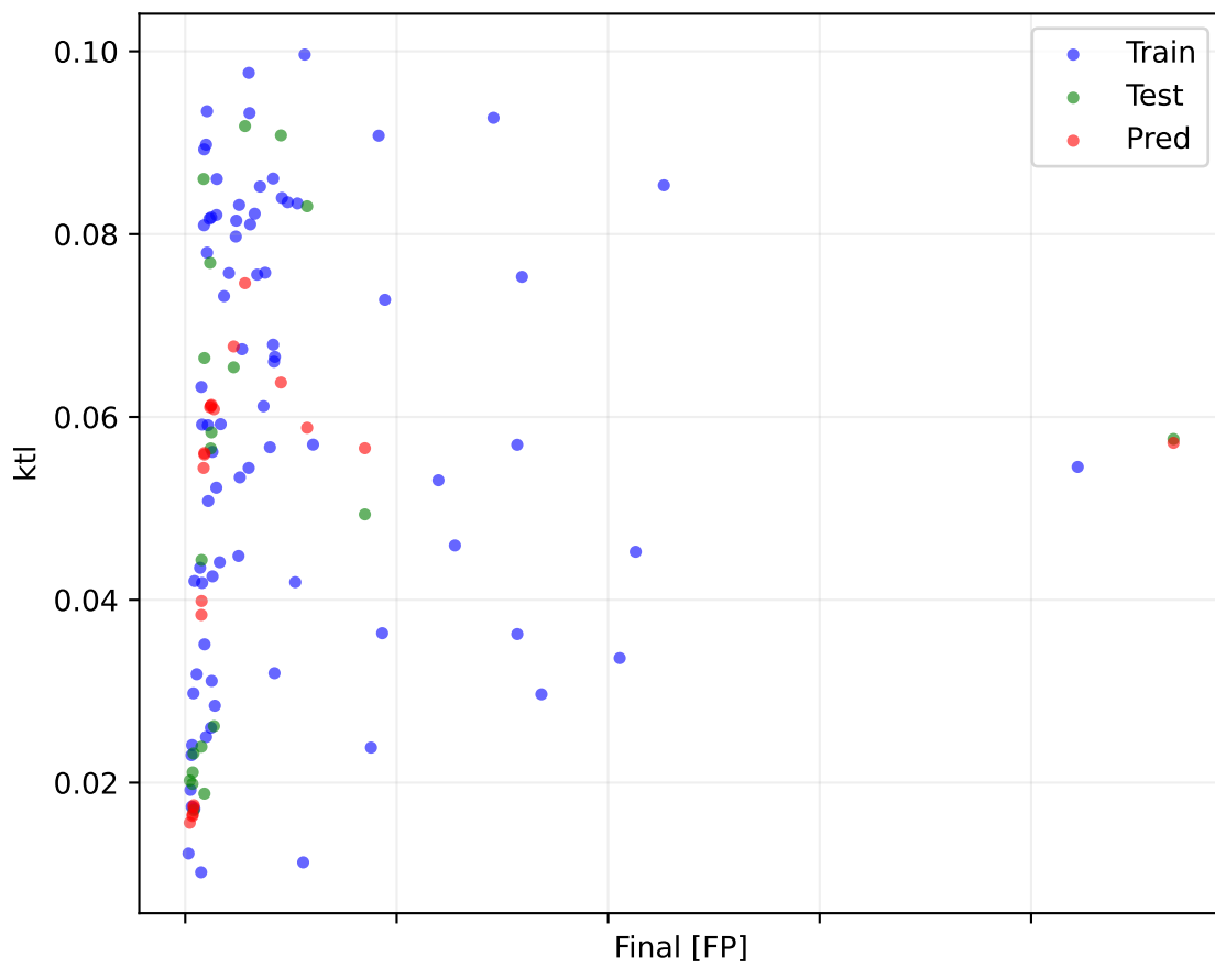
PILSTM Epoch 1000
