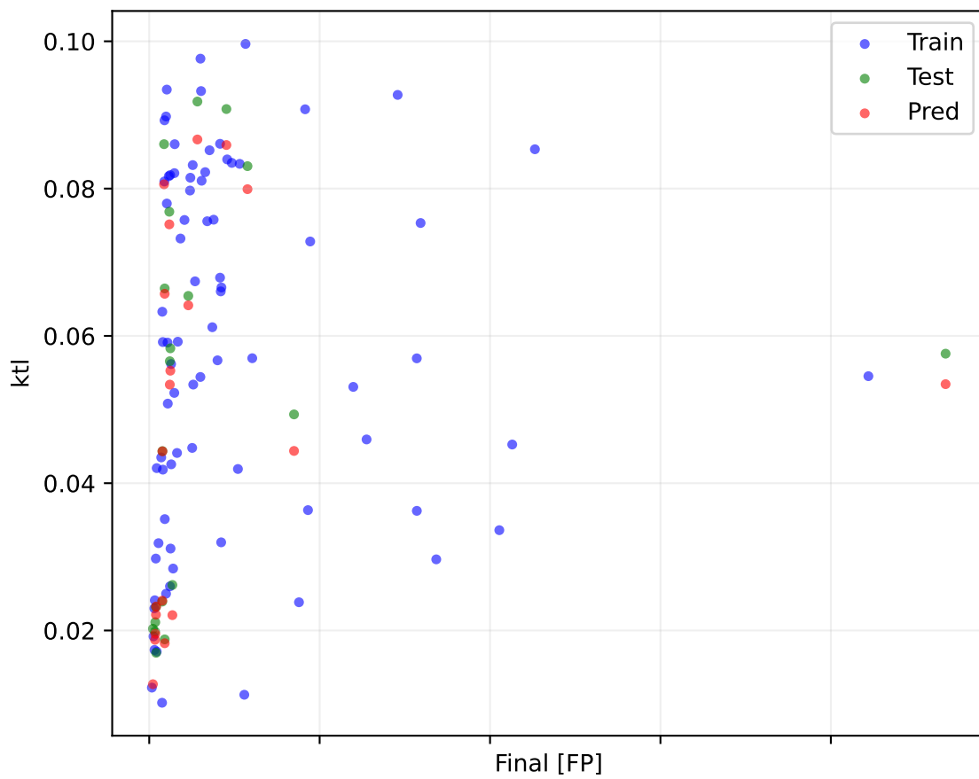
PILSTM Epoch 4000
