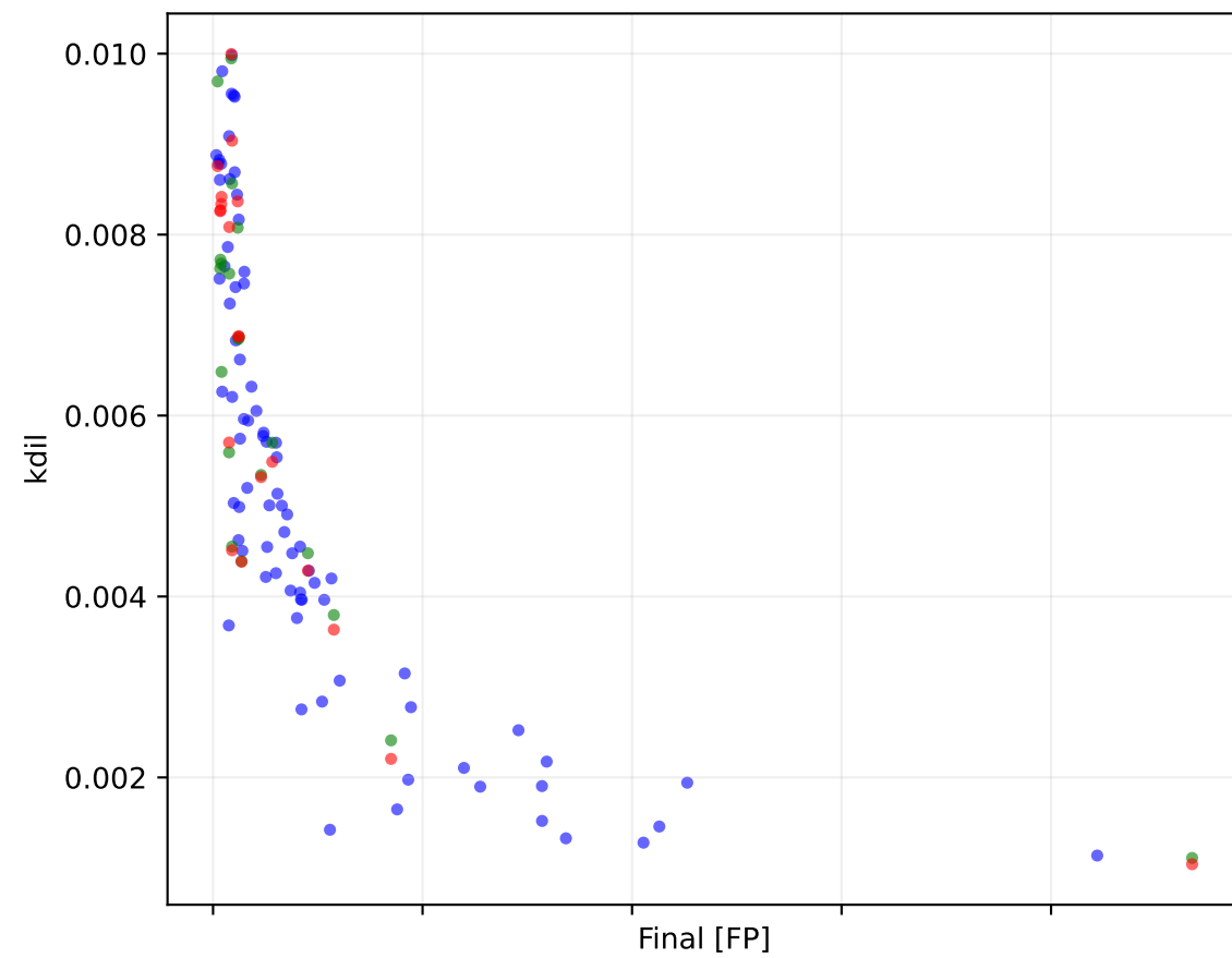
PILSTM Epoch 4000
