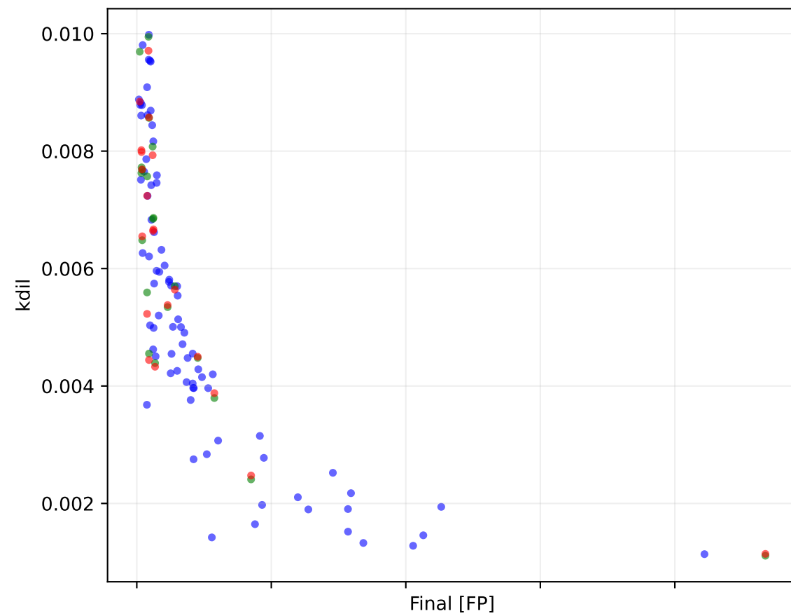
PILSTM Epoch 7000
