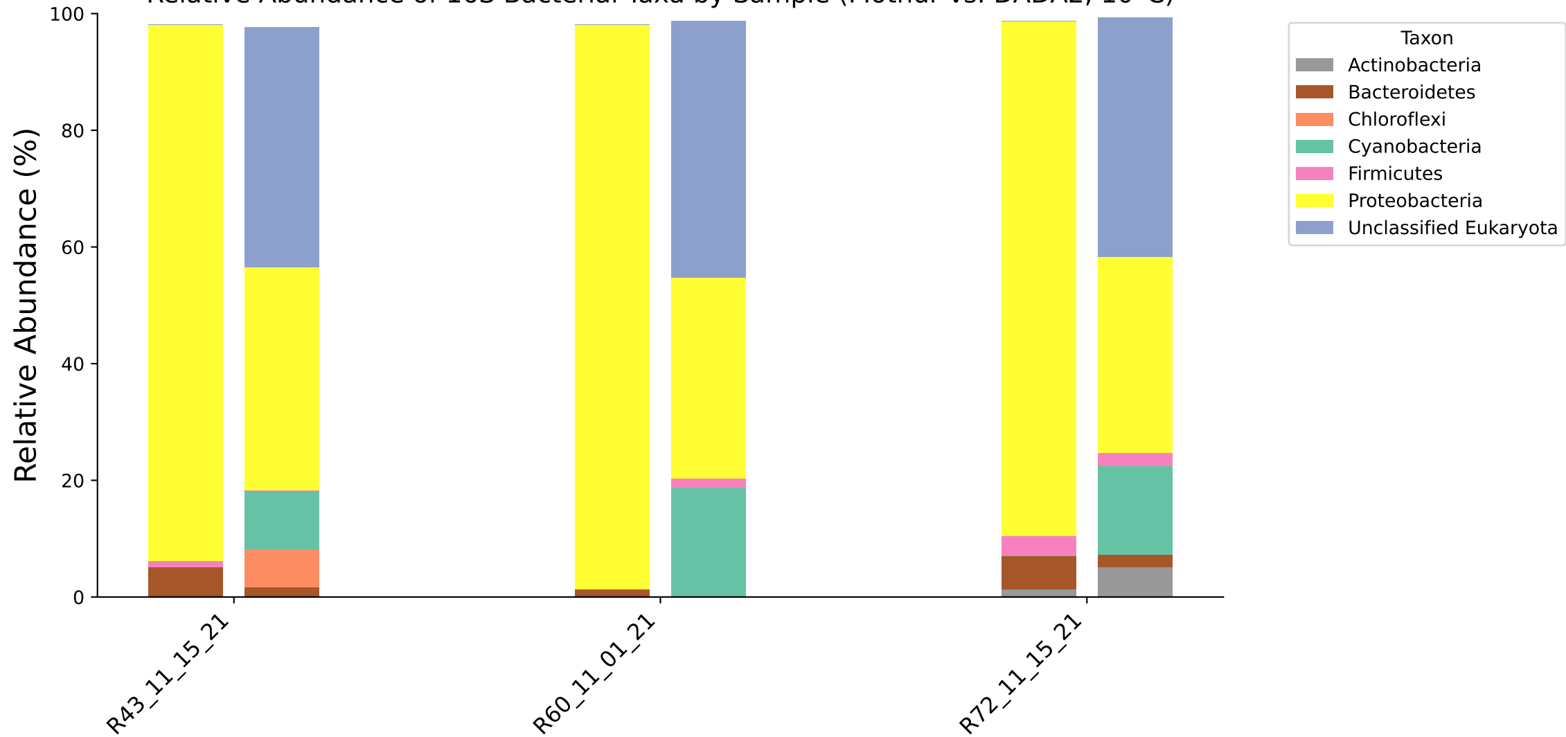
Relative Abundance of 16S Bacterial Taxa by Sample (Mothur vs. DADA2, 10°C)
