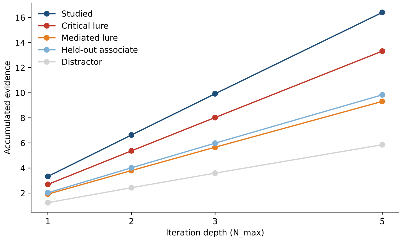
Accumulated recognition evidence by item type vs iteration depth (ConceptNet, 55 lists, 10 seeds)
