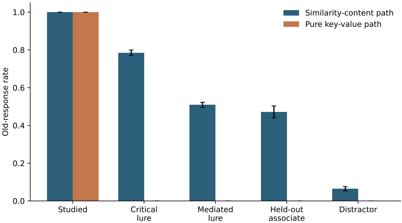
Dual-path dissociation: similarity-content vs pure key-value retrieval (ConceptNet, 55 lists, 20 seeds)
