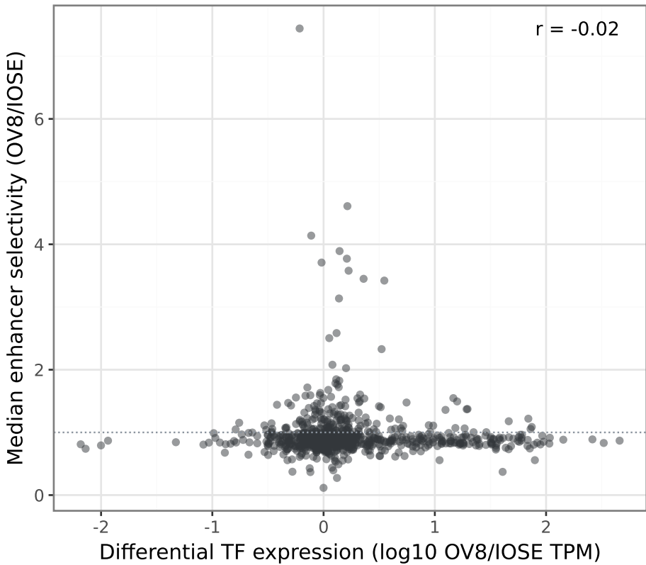
Current view: TF mRNA vs enhancer selectivity
