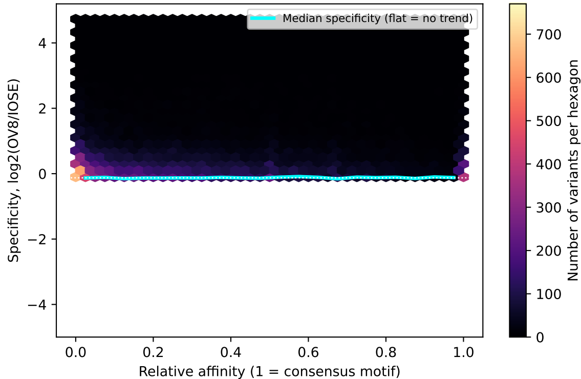
Specificity vs affinity — flat median = affinity doesn't predict specificity
