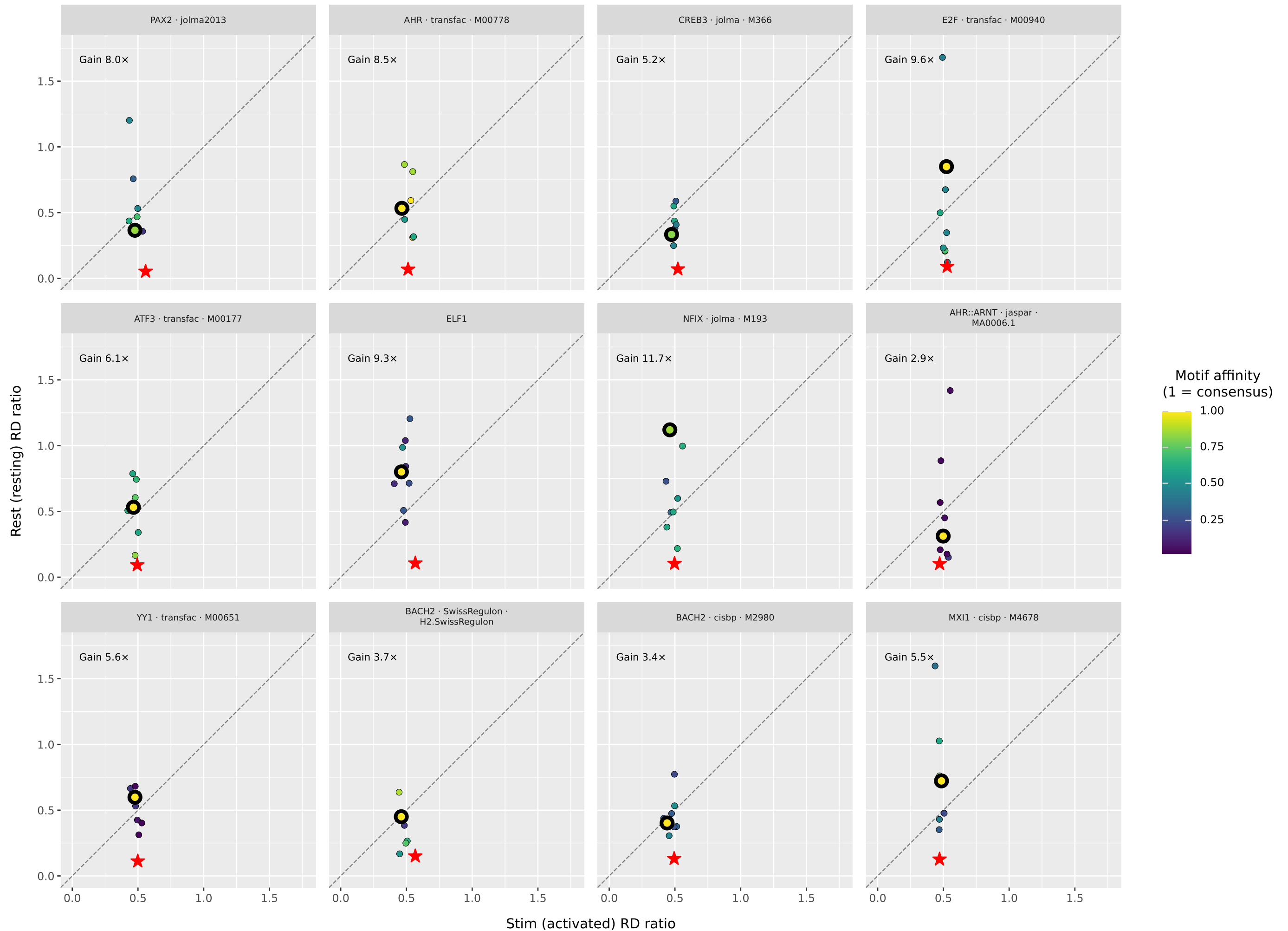
Per-PWM variant clouds — thick-edged dot = consensus, ★ = most-selective, below diagonal = stim-selective
