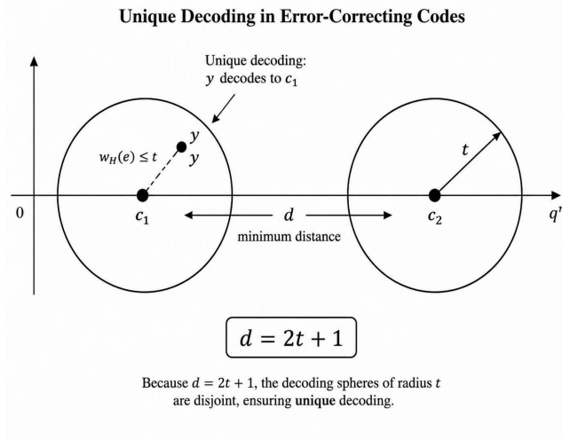
Figure 1.1: Unique decoding sphere visualization: if the minimum distance is d , then balls of radius t = \lfloor (d - 1)/2 \rfloor around each codeword are disjoint, ensuring unique decoding.
