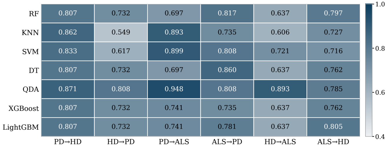
Cross-condition subject-level macro- F_1 by classifier and direction
