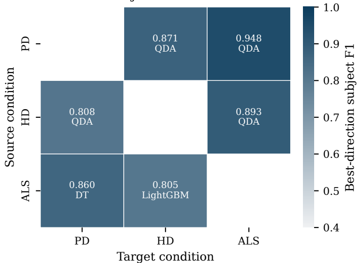
Best classifier and subject F1 for each transfer direction
