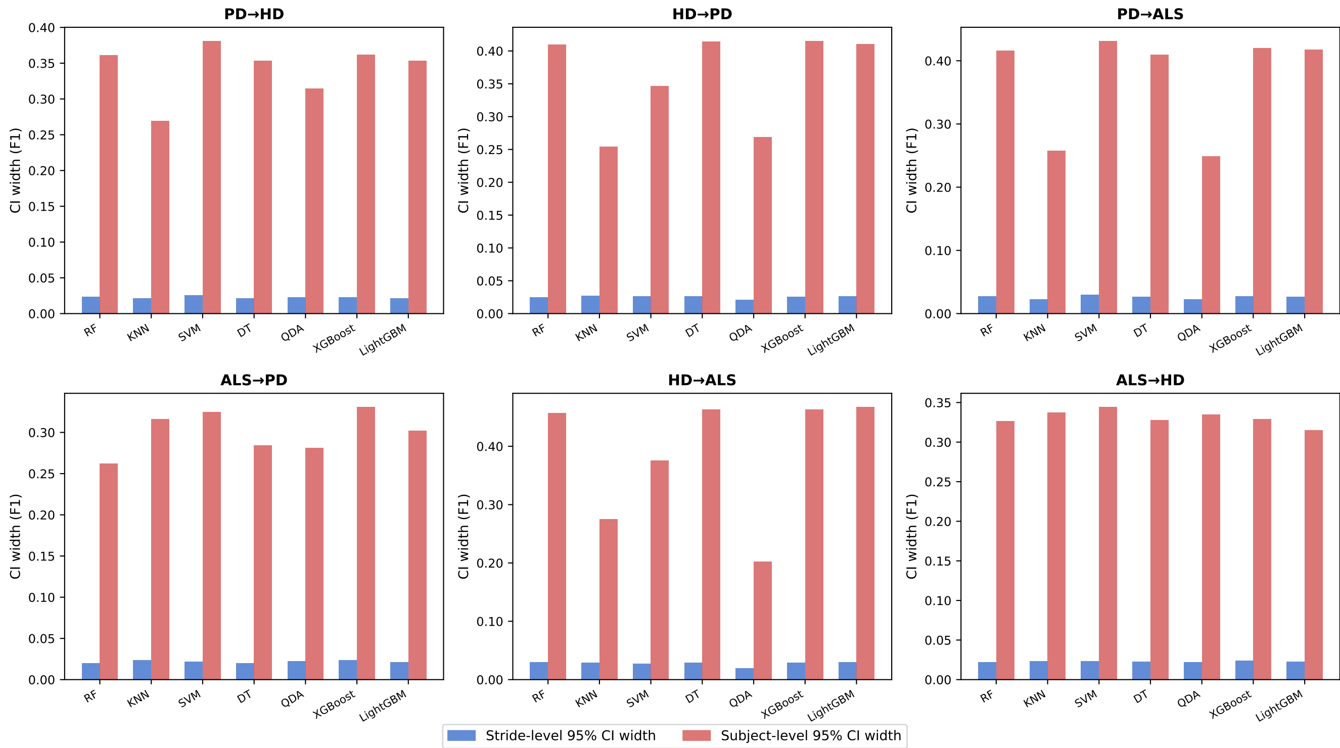
Bootstrap CI Width: Stride-Level vs. Subject-Level
