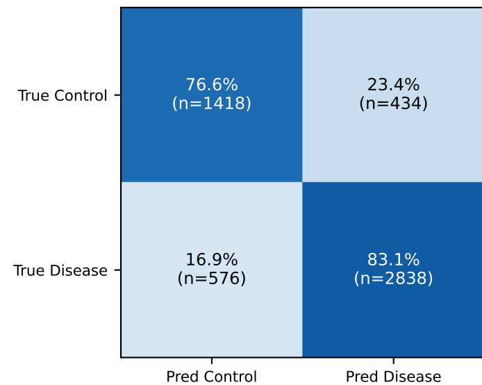
ALS→PD [SVM]
