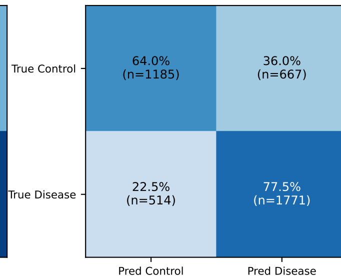
PD→ALS [RF]
