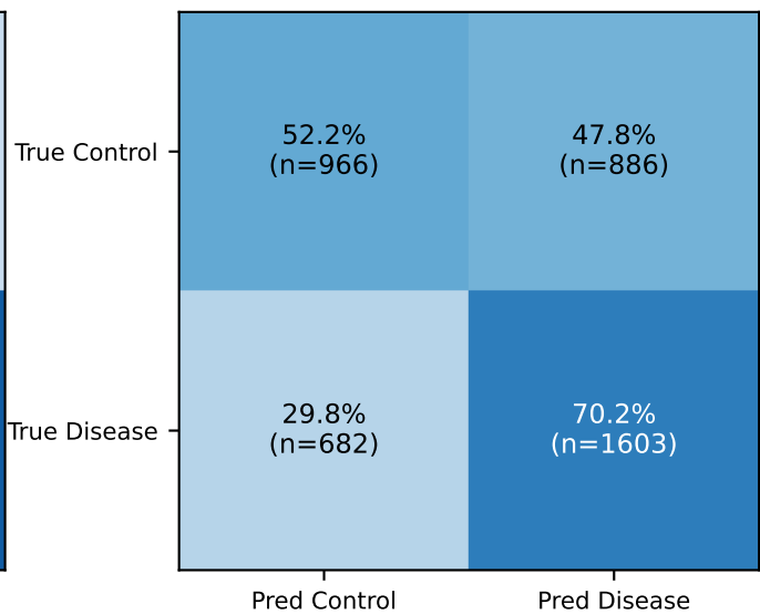
HD→ALS [XGB]
