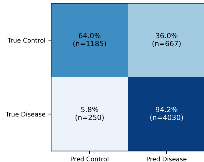
PD→HD [RF]
