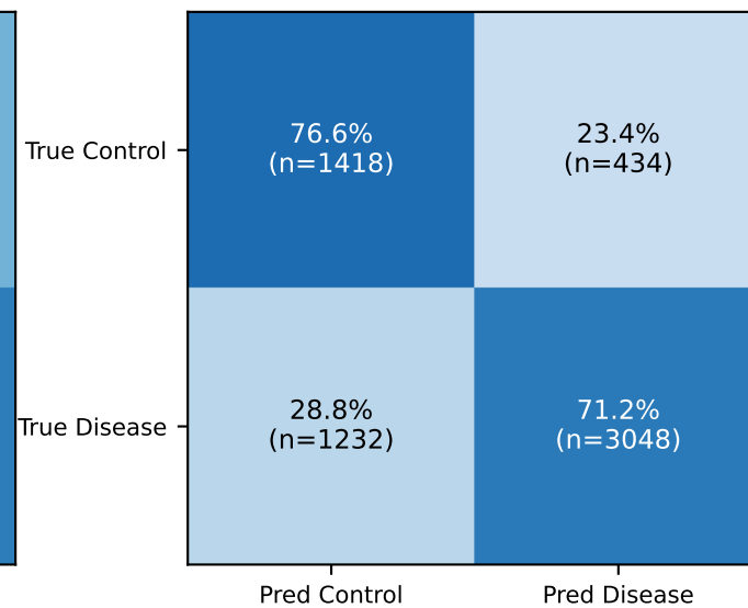
ALS→HD [SVM]
