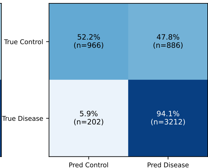
HD→PD [XGB]
