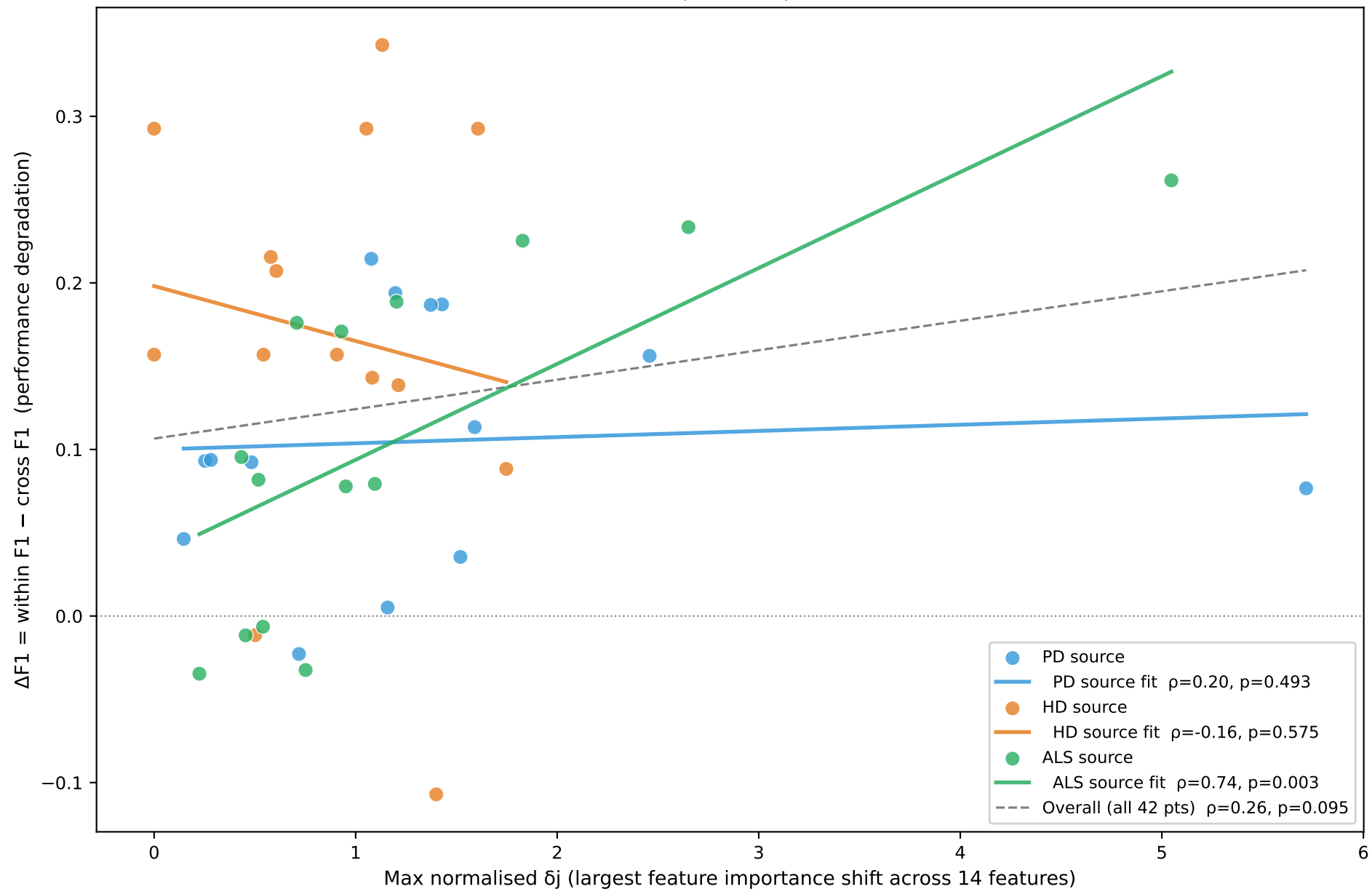
Feature Importance Shift vs Performance Degradation 42 (direction × classifier) pairs — Spearman rank correlation
