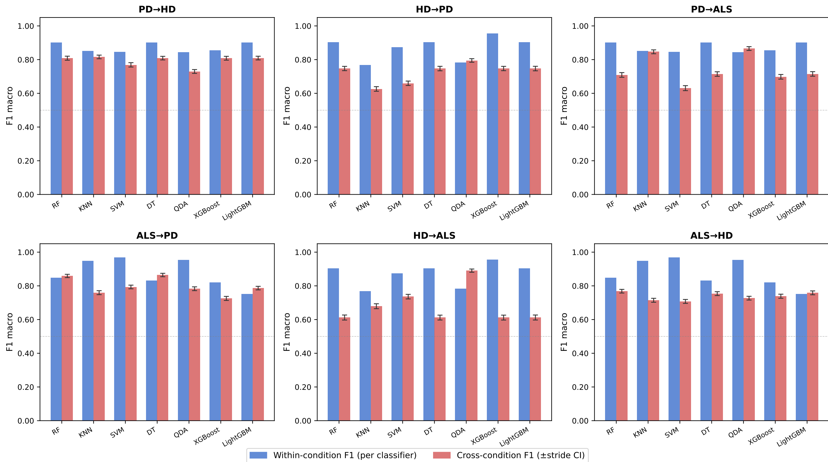
Within-Condition vs. Cross-Condition F1 by Classifier and Direction
