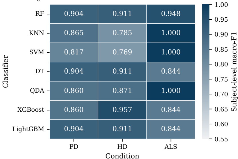
Subject-level macro-F1 across classifiers and conditions
