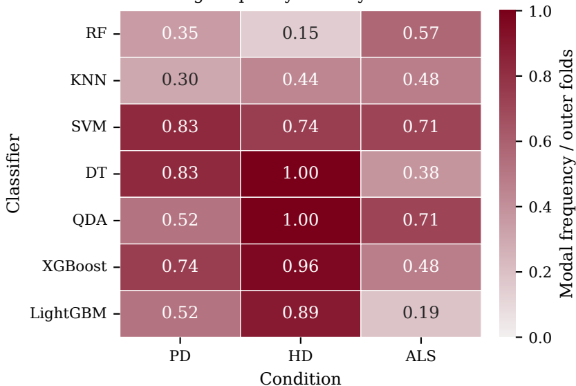
Modal winning-frequency stability across outer folds
