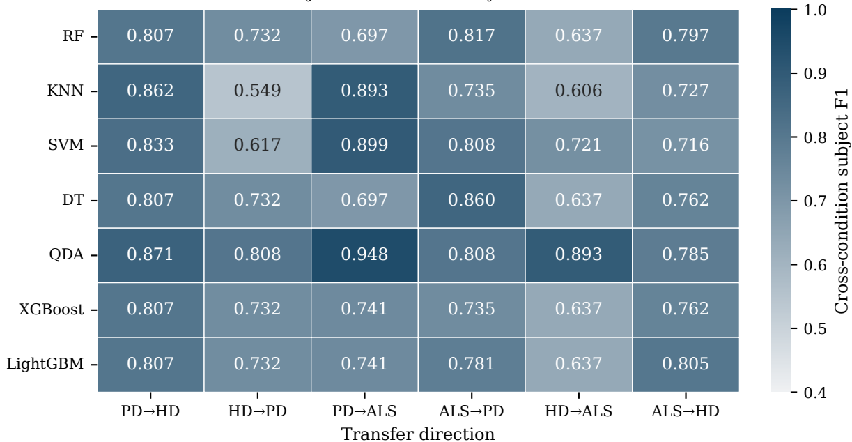
Cross-condition subject-level macro-F1 by classifier and direction
