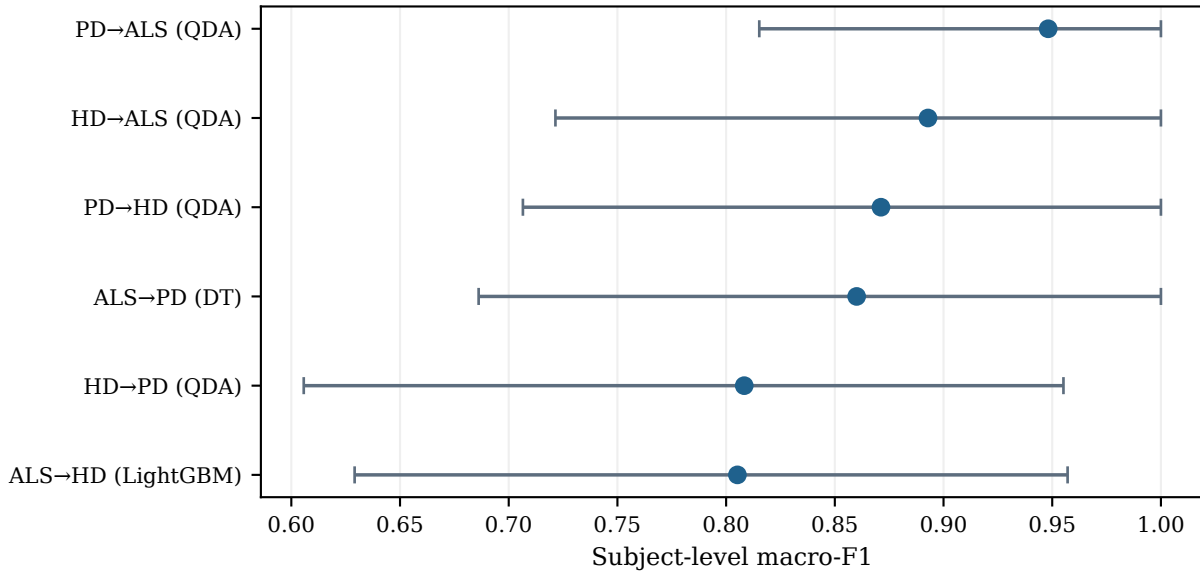
Best-direction bootstrap intervals
