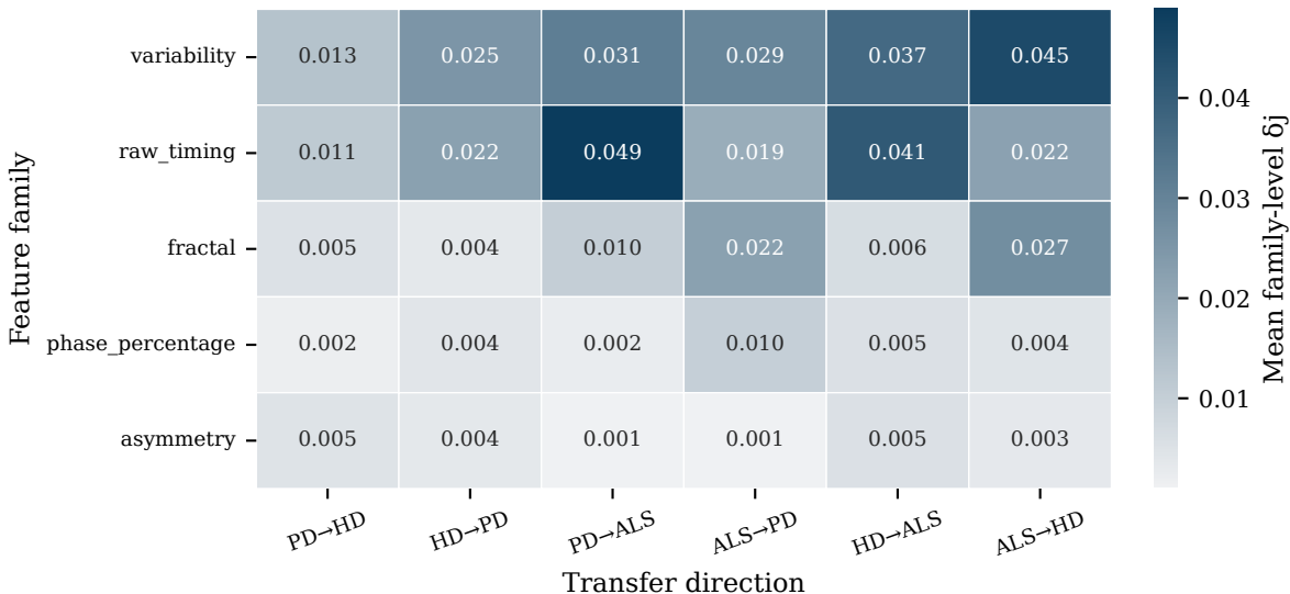
Feature-family consensus shift across transfer directions
