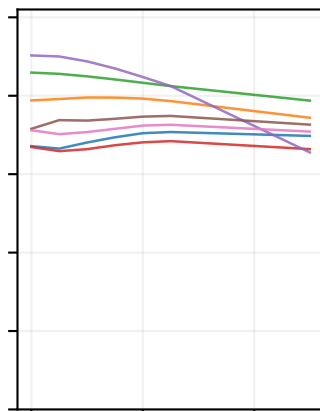
PD→ALS
