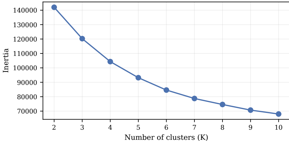
K-means elbow curve (stride-level v4 matrix)
