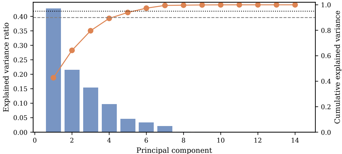
PCA explained variance (stride-level v4 matrix)
