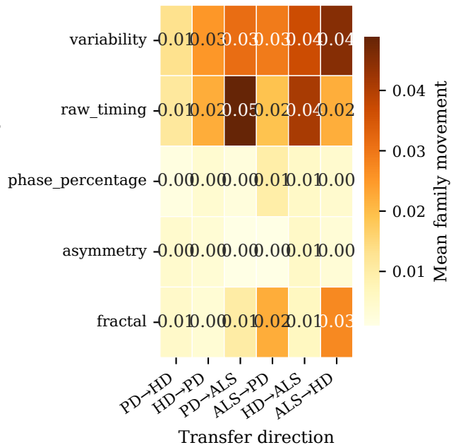
(b) Family-level movement consensus
