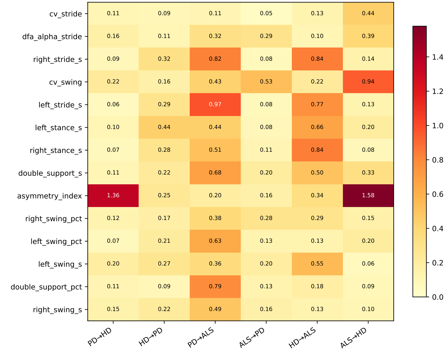
(B) Normalised \delta j — mean across 7 classifiers
