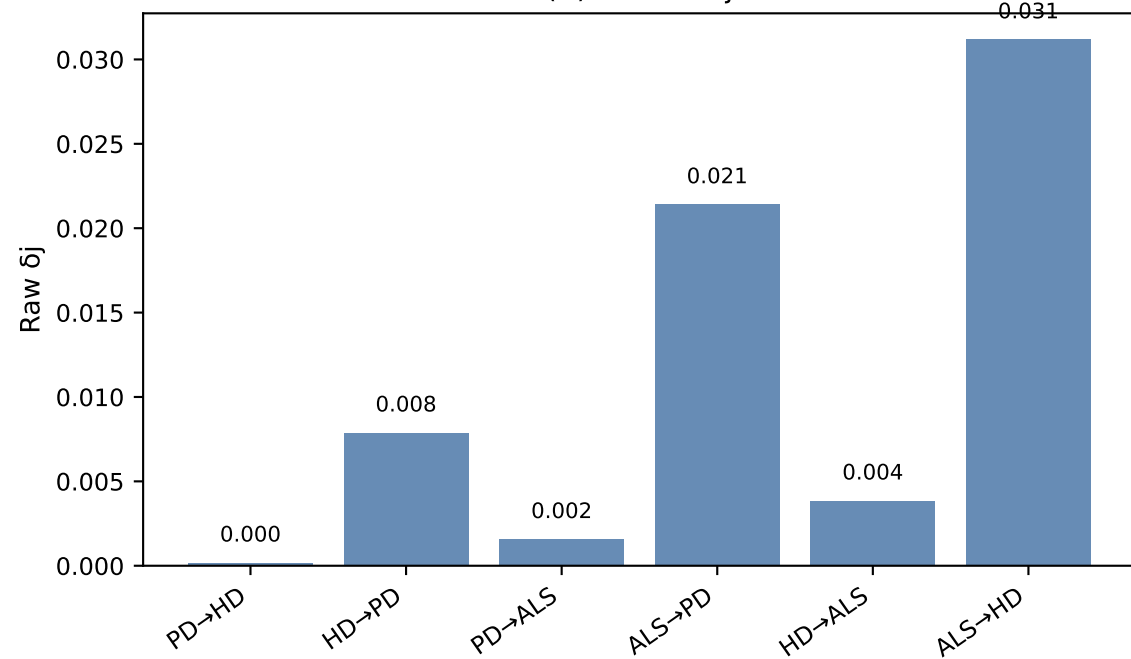
(A) RF raw \delta j
