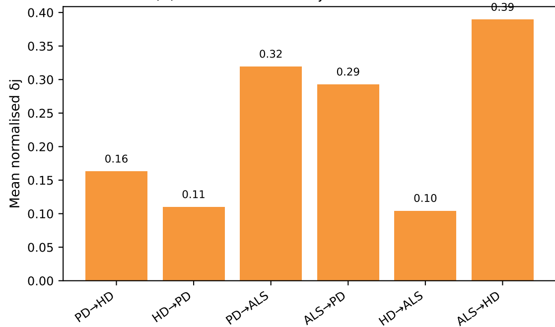
(B) Mean normalised \delta j across 7 classifiers
