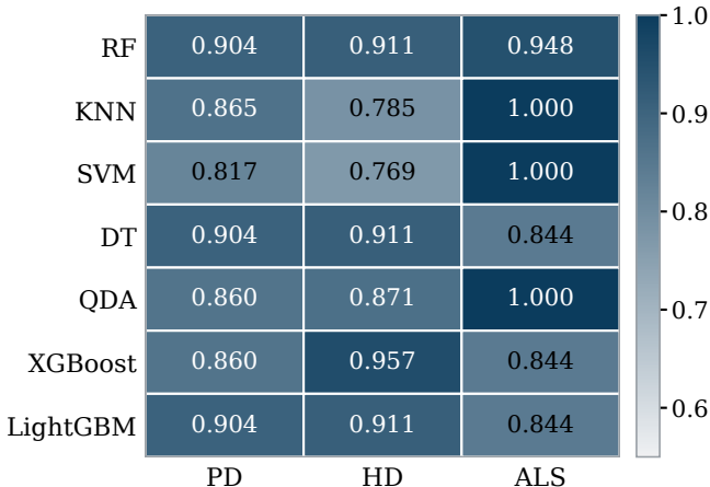
Within-condition subject-level macro- F_1
