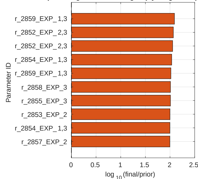
Top 10 Largest Kcat Changes (by magnitude)
