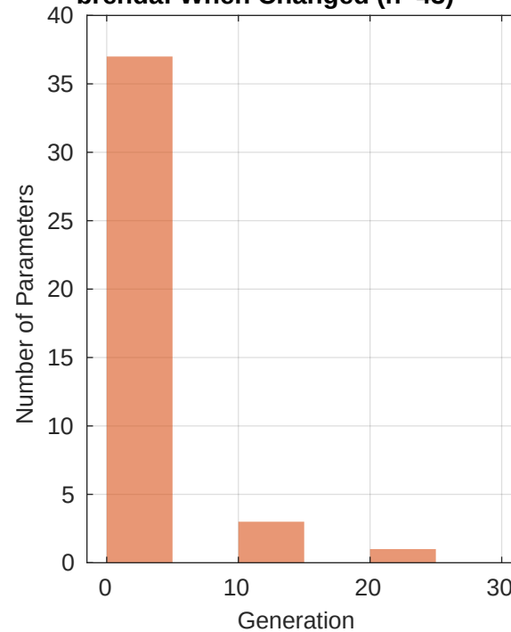
brenda: When Changed (n=43)
