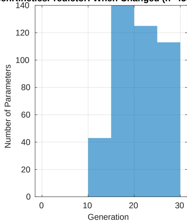
OpenKineticsPredictor: When Changed (n=459)
