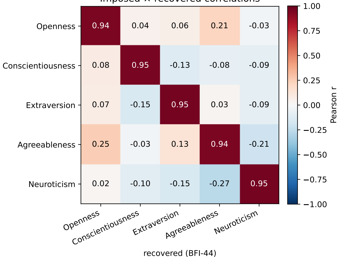
Imposed × recovered correlations
