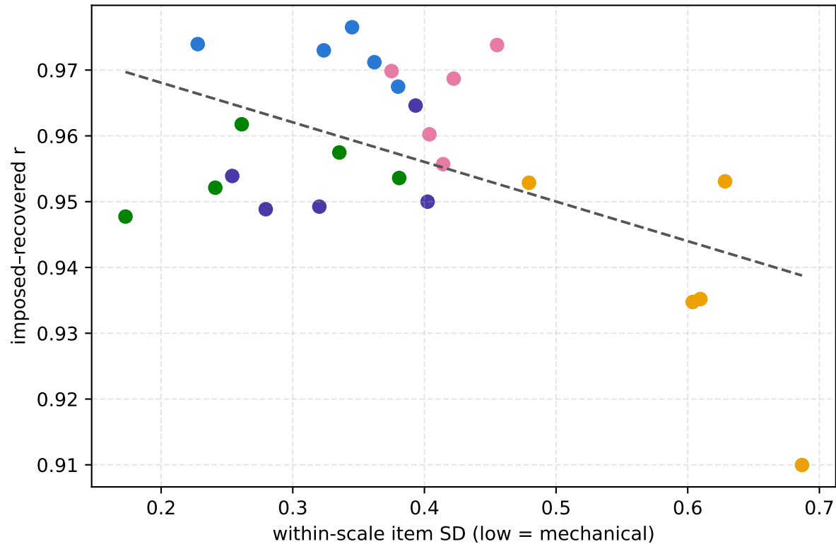
Within-scale variability vs recovery ( r = -0.52 , 25 cells)
