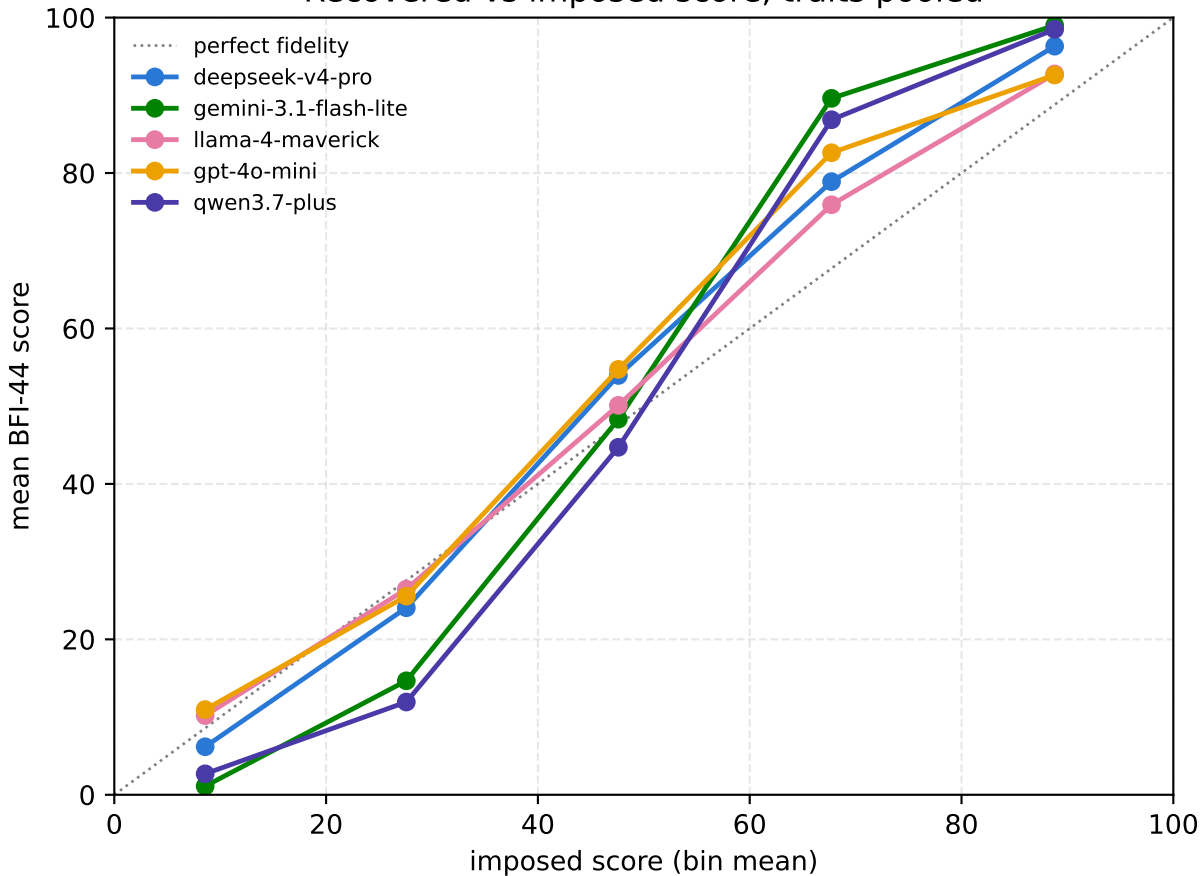
Recovered vs imposed score, traits pooled
