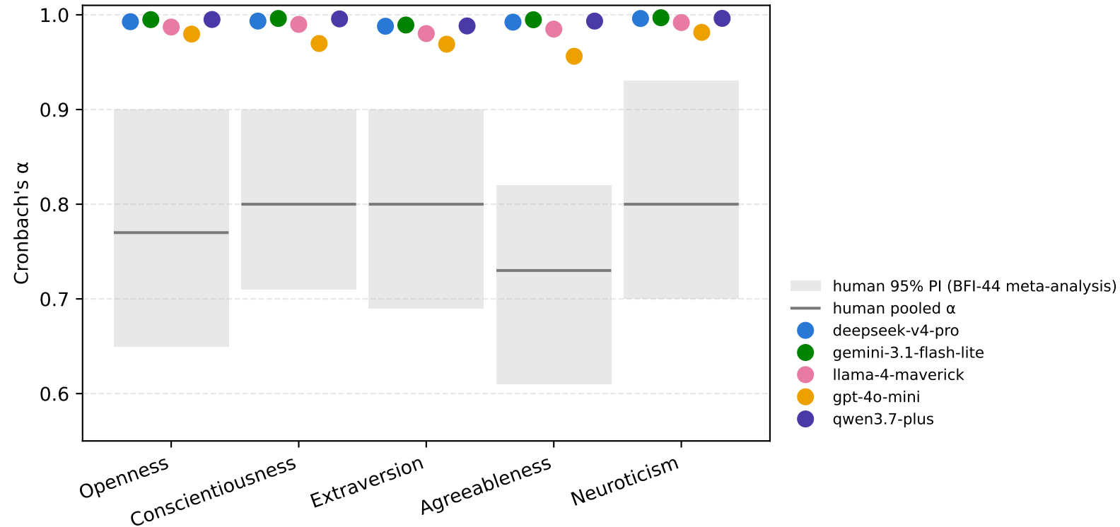
Internal consistency by model and trait
