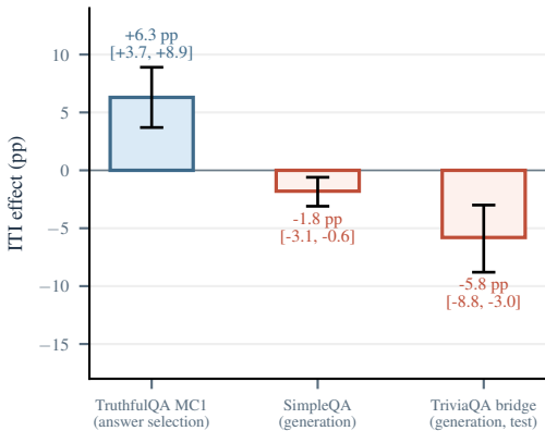
(a) ITI: surface-local gain, generation harm
