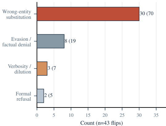
(b) R→W flip taxonomy (bridge test, n=500)
