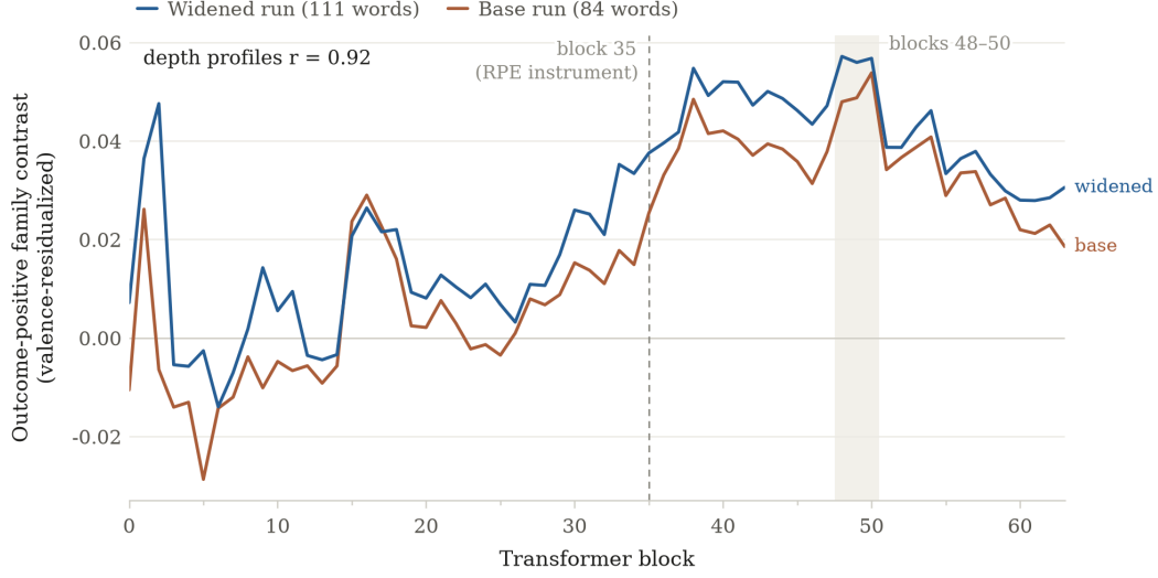
Figure 4. Depth profile of the outcome-positive family contrast (valence-only design) across transformer blocks for the base and widened runs ( r = 0.92 ). Dashed line: block 35, where the RPE direction is read; shaded band: blocks 48–50, where the contrast peaks in both runs.
