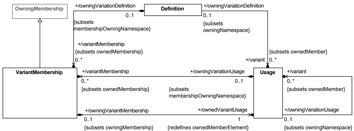
Figure 9. Variant Membership
