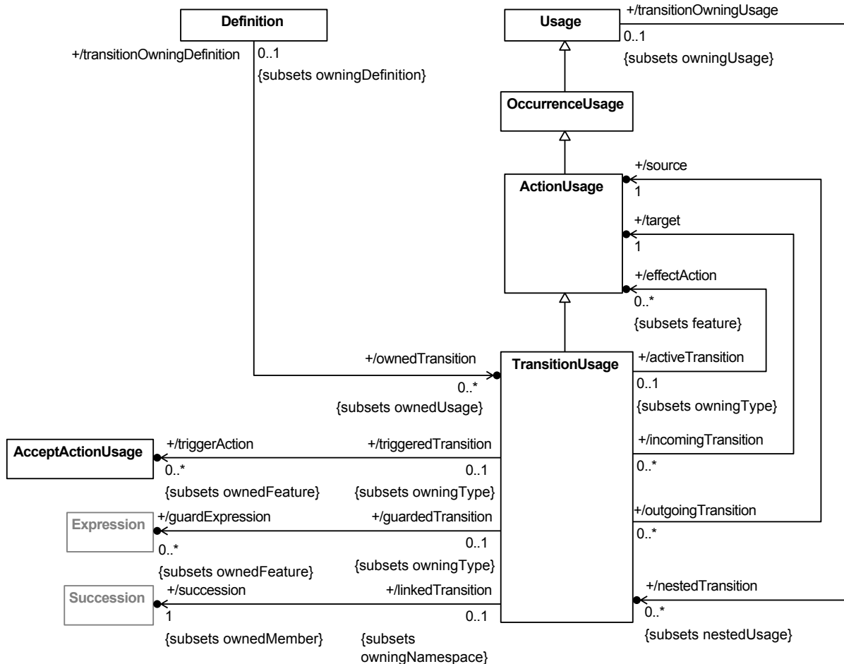
Figure 33. Transition Usage
