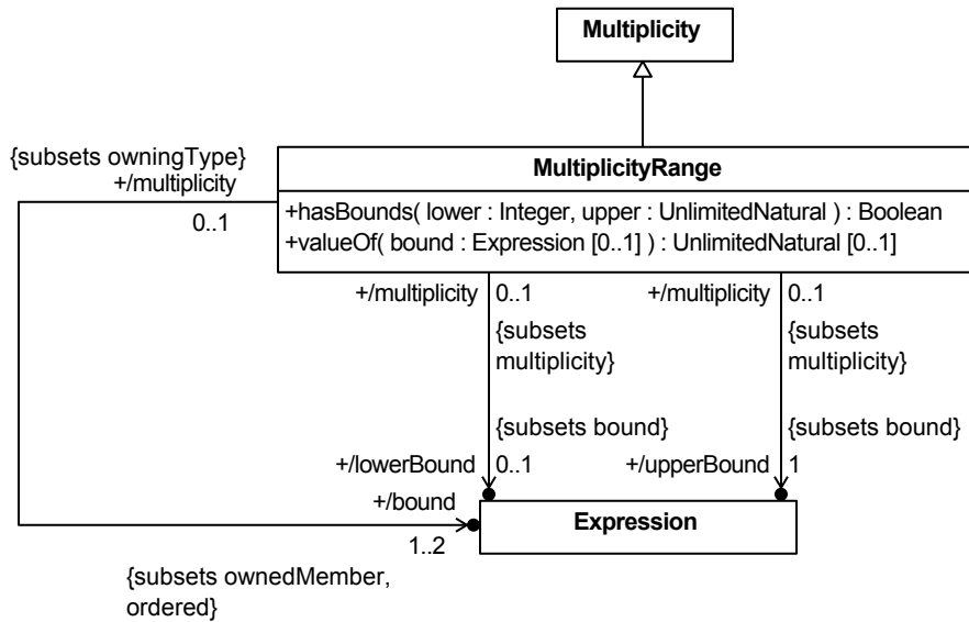
Figure 38. Multiplicities
