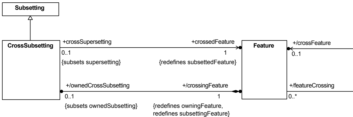
Figure 22. Cross Subsetting
