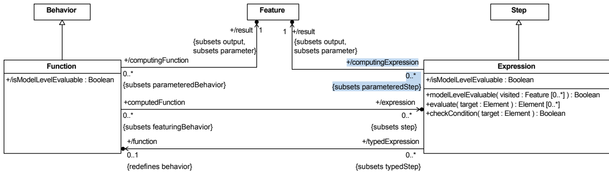
Figure 30. Functions
