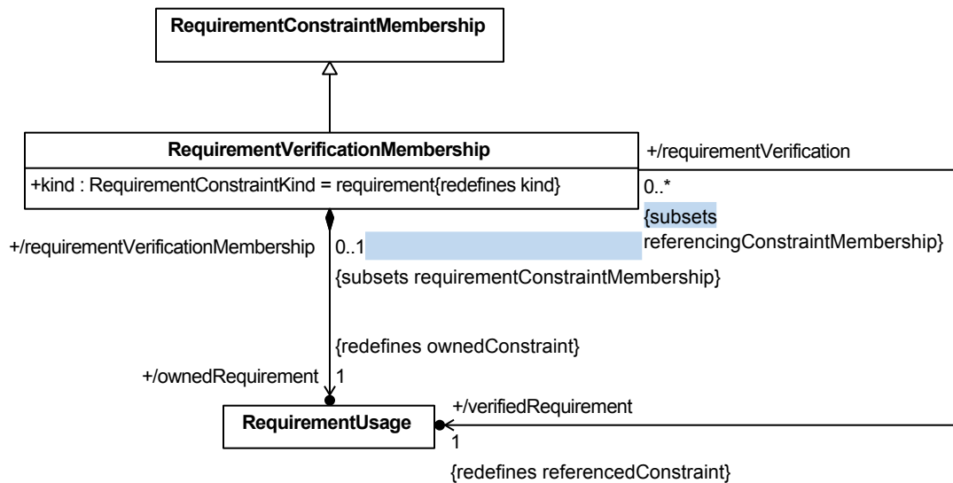
Figure 46. Verification Membership
