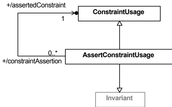
Figure 36. Asserted Constraints
