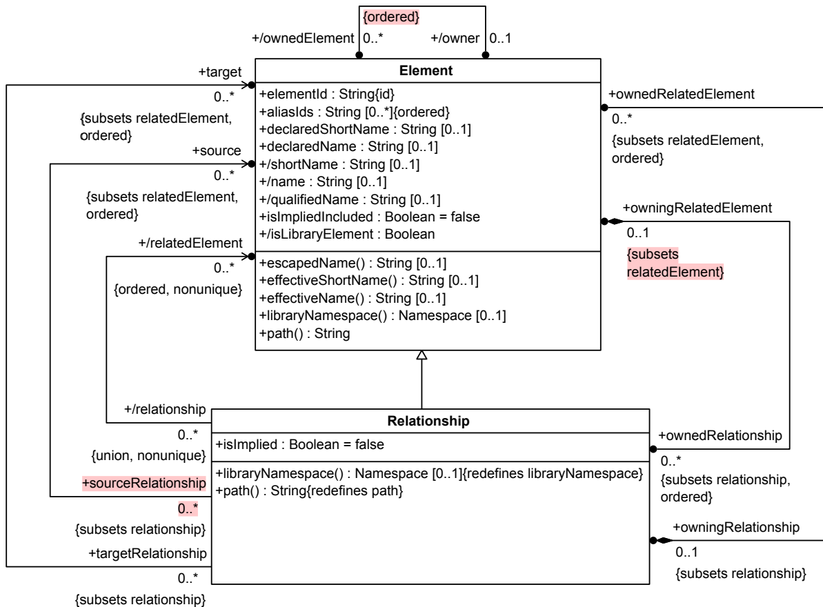
Figure 2. Elements
