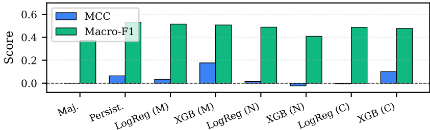
Test Performance (MCC & Macro-F1)
