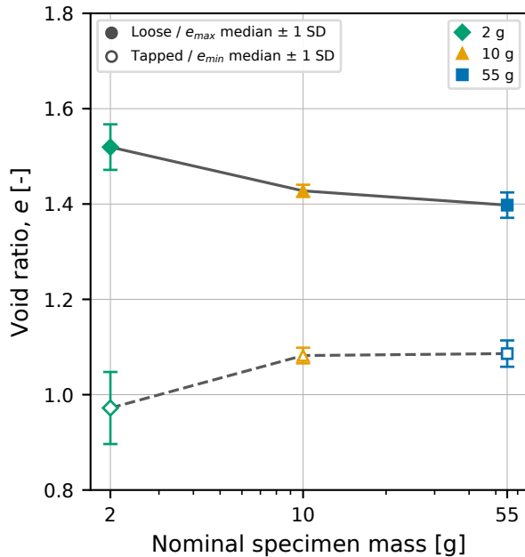
Void ratio
