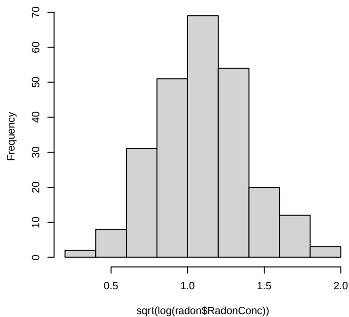
Histogram of \sqrt{\log(\text{radon}\$RadonConc)}
