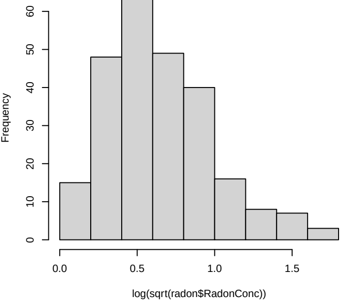
Histogram of \log(\sqrt{\text{radon}\$RadonConc})
